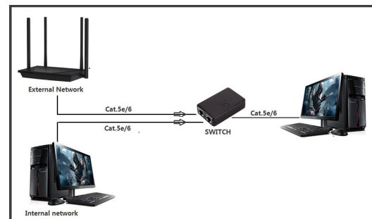
K9131C/1 2 IN 1 SWITCHET INTERNAL AND EXTERNAL NETWORK SWITCHING NETWORKING
