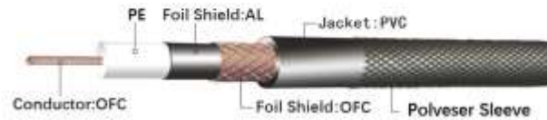
K7009BD-RB 6.3mm Mono Male To 6.3mm Mono Male Metal Shell Mic Cable Double Shielded 60% OD:6mm Black Soft Cable + Red/Black Polyester Sleeve
