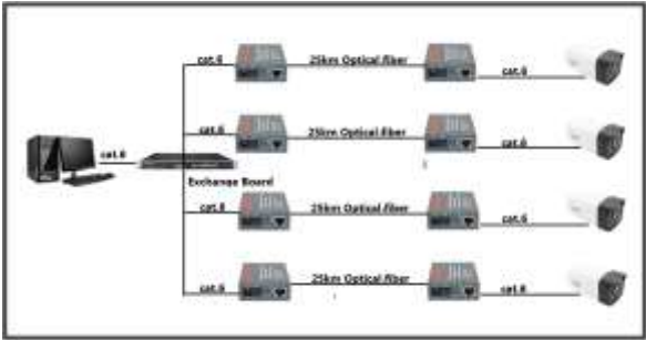
K8360TE11A 1P Network optoelectronic converter, optical fiber transceiver
