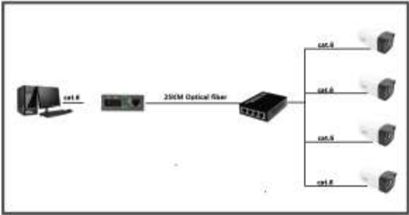
K8360TE14A 4P Network optoelectronic converter, optical fiber transceiver
